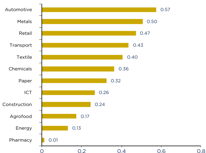
Chart 9 Correlation coefficient between GDP growth and added value growth of 12 business sectors between 1985 and 2016 (average of 15 countries)
